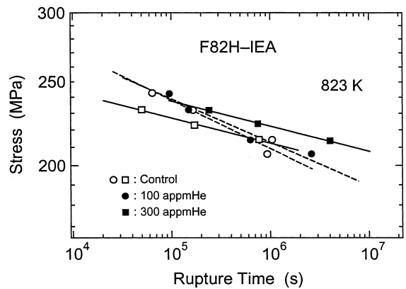
Fig. 2. A plot of creep stress vs time to rupture for helium implanted ( C_{He} = 100 and 300 appm) and unimplanted F82H IEA heat material tested at 823 K.
