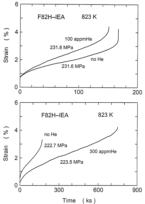
Fig. 1. Creep strain-time recordings of IEA modified F82H in helium implanted ( C_{He} = 100 and 300 appm) and unimplanted conditions.
